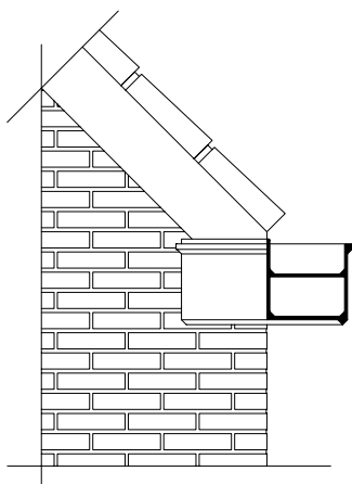
Detail 250.08
