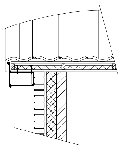
Detail 250.14
