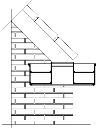
Detail 250.08A
